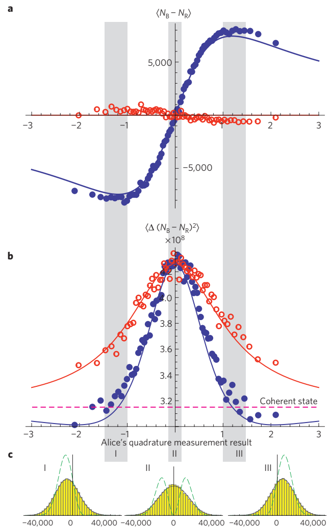
Figure 2 | Photon number statistics of the state in Bob's channel that is conditionally prepared by Alice's quadrature measurement. a, b , Mean (a) and variance (b) of the difference N_B - N_R between the photon numbers and the reference beam. Filled circles correspond to the displacement in Bob's channel along the same quadrature as Alice's measurement; for open circles the displacement and measurement are in orthogonal quadratures. The dashed line in b corresponds to 2\alpha^2 ; that is, the variance that would be observed if Bob's channel contained a coherent state of amplitude \alpha . c, Histograms of N_B - N_R conditioned on Alice's measurement result within intervals I, II, III shown in a, b by shaded areas. All histograms correspond to the displacement and measurement in the same quadrature. Solid and dashed lines in c show theoretical predictions, respectively with and without taking experimental imperfections into account. The statistics represented by histograms I and III, corresponding approximately to states 1/\sqrt{2}\hat{D}(\alpha)(|0\rangle \pm |1\rangle) , can be distinguished by a single energy measurement with a 68% certainty. They are reminiscent of the dead and alive states of Schrödinger's cat.
